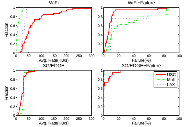
Figure 4: (CDF) Link availability with failure probability
